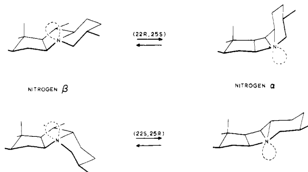
Figure 3. Solanidan conformers produced by nitrogen inversion.
